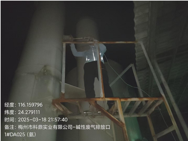
碱性废气排放口 1#DA025: 氨
